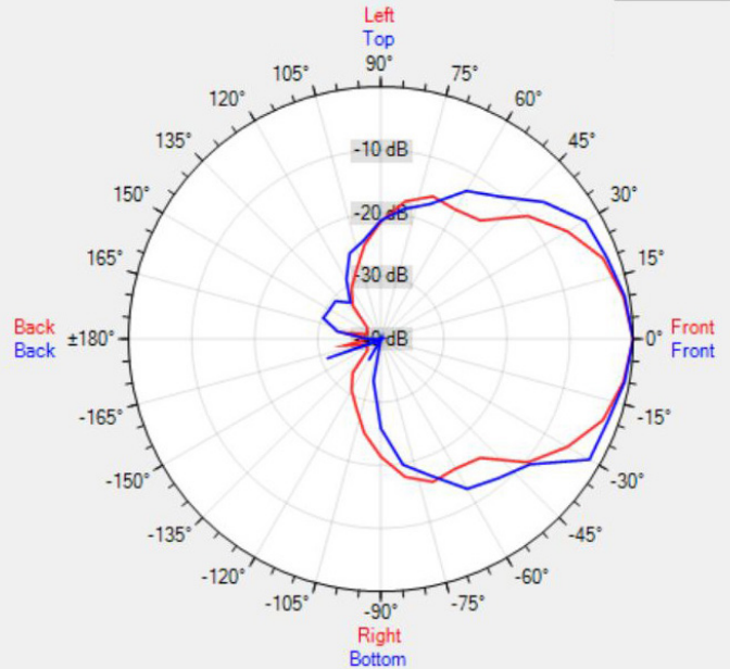
Data Shown: MASK12-70x90 (Apart Audio) Display Parameters: Frequency: 8000Hz (1/24th Octave)
