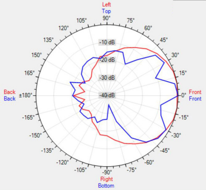
Data Shown: MASK12-90x70 (Apart Audio) Display Parameters: Frequency: 2000Hz (1/24th Octave)
