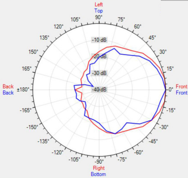
Data Shown: MASK12-90x70 (Apart Audio) Display Parameters: Frequency: 4000Hz (1/24th Octave)
