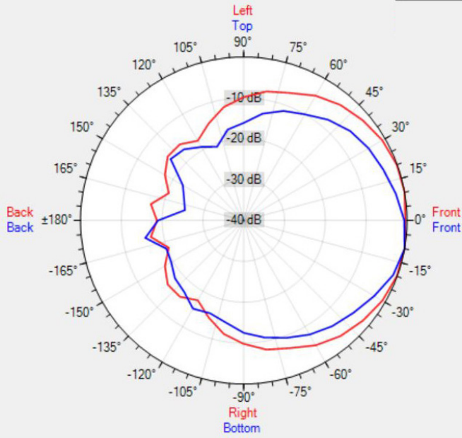
Data Shown: MASK12-90x70 (Apart Audio) Display Parameters: Frequency: 1000Hz (1/24th Octave)
