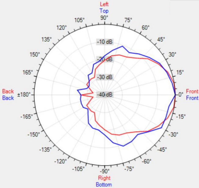
Data Shown: MASK12-70x90 (Apart Audio) Display Parameters: Frequency: 4000Hz (1/24th Octave)
