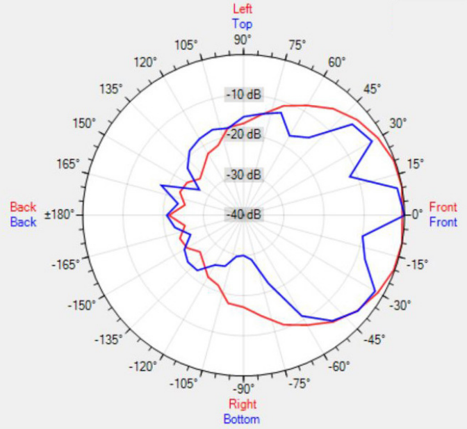
Data Shown: MASK12-70x90 (Apart Audio) Display Parameters: Frequency: 2000Hz (1/24th Octave)
