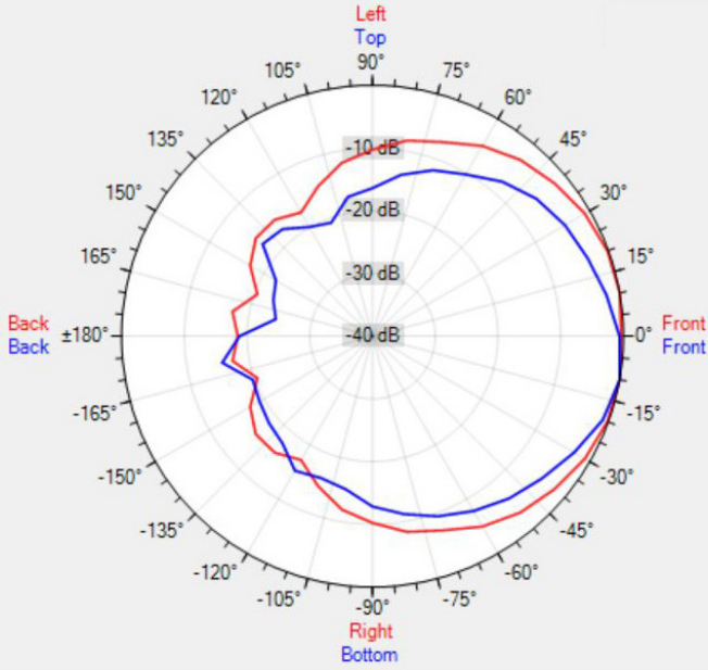
Data Shown: MASK12-70x90 (Apart Audio) Display Parameters: Frequency: 1000Hz (1/24th Octave)
