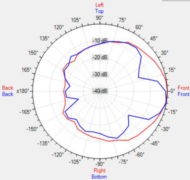
Data Shown: OVO3 (Apart Audio) Display Parameters: Frequency: 4000Hz (1/24th Octave)
