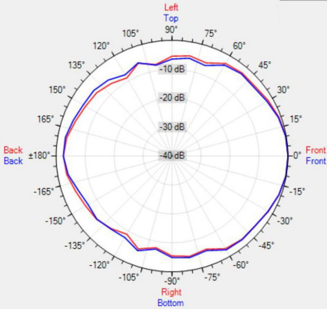
Data Shown: OVO3 (Apart Audio) Display Parameters: Frequency: 1000Hz (1/24th Octave)
