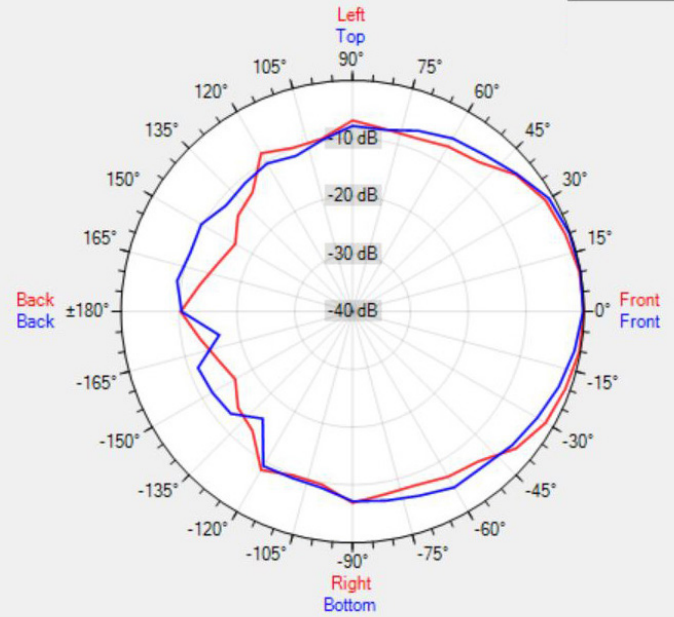
Data Shown: OVO3 (Apart Audio) Display Parameters: Frequency: 2000Hz (1/24th Octave)
