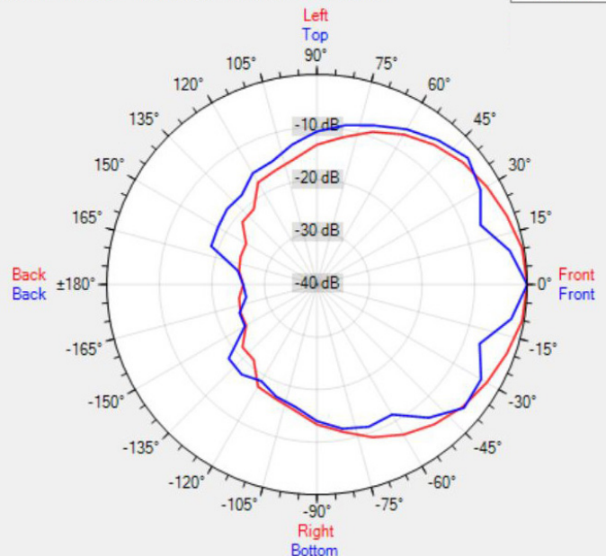
Data Shown: OVO3 (Apart Audio) Display Parameters: Frequency: 8000Hz (1/24th Octave)
