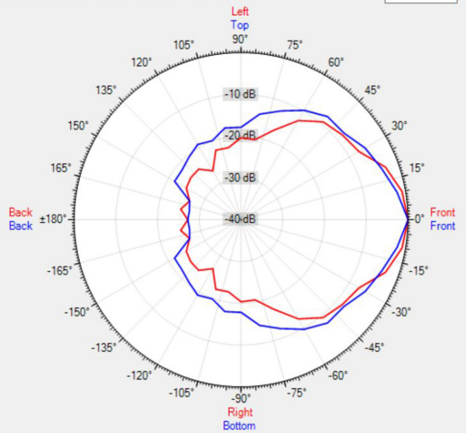
Data Shown: KUBO5T (Apart Audio) Display Parameters: Frequency: 8000Hz (1/24th Octave)
